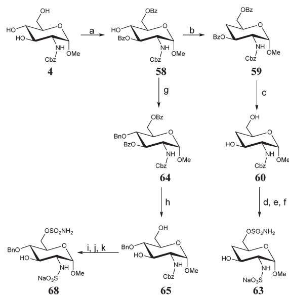
Scheme 6 Reagents and conditions: (a) \text{BzCl} (2.2 eq.), \text{CH}_2\text{Cl}_2 -pyridine, -40^\circ\text{C} , 3 h, 72%; (b) (i) \text{CS}(\text{Im})_2 , toluene, 110^\circ\text{C} , 3 h; (ii) \text{TMS}_3\text{SiH} , AIBN, 110^\circ\text{C} , 1 h, 79%; (c) \text{NaOMe} (cat), MeOH, r.t., 18 h, 68%; (d) \text{ClSO}_2\text{NH}_2 , DMF, -40^\circ\text{C} , 36 h, 51%; (e) \text{H}_2/10\% Pd/C, AcOH, 40^\circ\text{C} , 2 h, 70%; (f) \text{SO}_3\cdot\text{Py} , \text{H}_2\text{O} , pH 9–10, r.t., 2 h, 8%; (g) benzyl-2,2,2-trichloroacetimidate (8 eq.), TfOH, dioxane, 60^\circ\text{C} , 4 h, 78%; (h) 3 eq. \text{LiAlH}_4 , 0^\circ\text{C} , 2 h, 69%; (i) \text{ClSO}_2\text{NH}_2 , Tol-DMA, -40^\circ\text{C} , 22 h, 52% (j) 10 bar \text{H}_2/5\% Pd/C, MeOH, r.t. 35 min, 100% (k) \text{SO}_3\cdot\text{Py} , \text{H}_2\text{O} , pH 9–10, r.t., 2 h, 25%.
