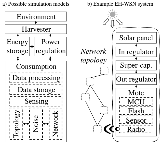
Figure 1: (a) Stack of simulation models (arrows denote possible model interactions) (b) An example EH-WSN setup (arrows denote energy flow)
