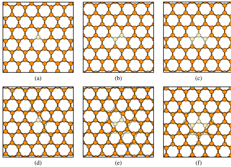
Figure 2. Model vacancy structures in bilayer graphene viewed along the prismatic direction where the atoms in the nearer layer are shown in a darker shade than those behind. Unoptimized models for (a) monovacancy, (b) divacancy and (c) trivacancy. Optimized structures for (d) monovacancy, (e), divacancy and (f) trivacancy.
