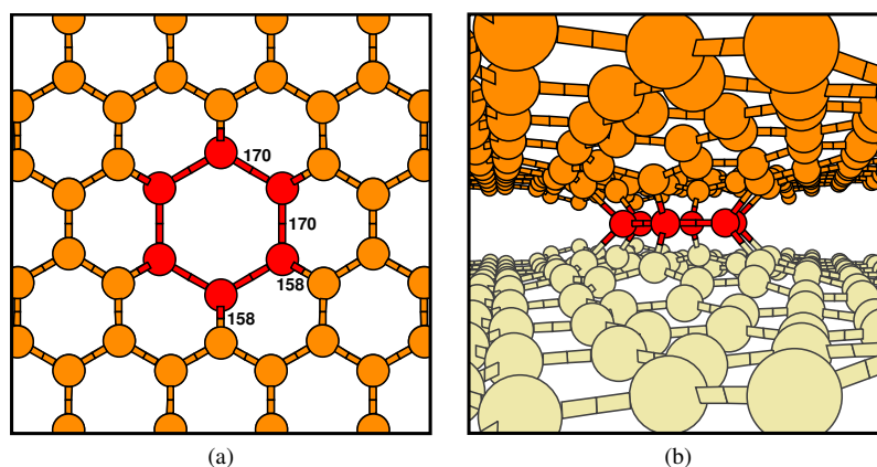
Figure 5. Geometry optimized structure of V_3 - V_3 mezzanine defect structure: (a) view along the prismatic axis (b) view along the basal plane. Bond lengths marked in picometres.
