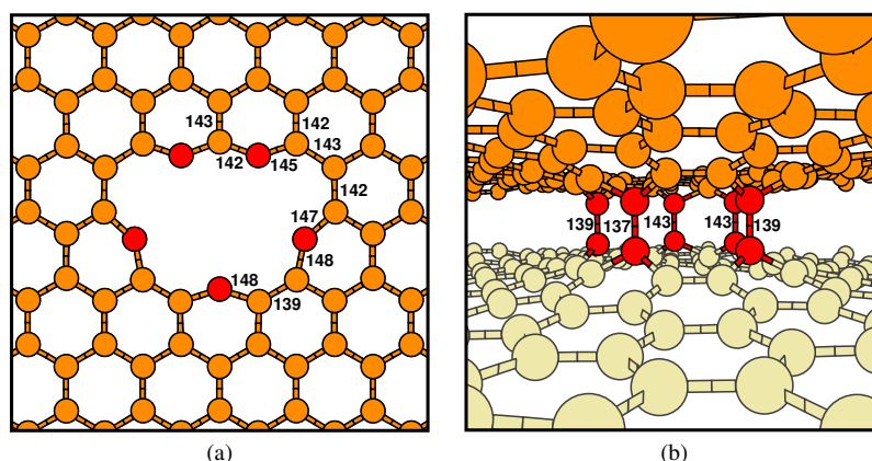
Figure 4. Geometry optimized structure of V_3 - V_3 wormhole defect structure: (a) view along the prismatic axis (b) view along the basal plane. Bond lengths marked in picometres.
