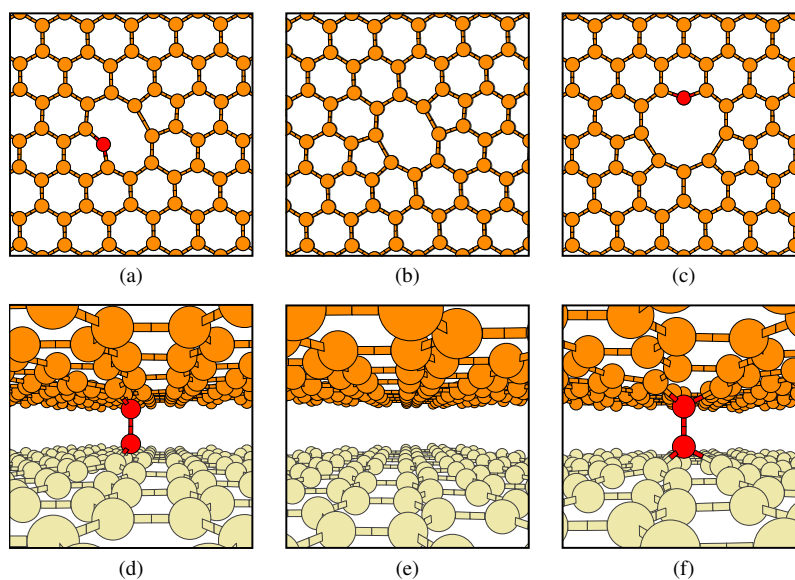
Figure 3. Geometry optimized AA-stacked bilayer graphene complexes of in plane view (a) divacancy species V_1-V_1 with one sp^2 interlayer bond, (b) tetravacancy species, V_2(5-8-5)-V_2(5-8-5) (no interlayer sp^2 bonds), (c) hexavacancy species V_3-V_3 with one sp^2 interlayer bond and its out of plane view in (d), (e) and (f). The red atom has an sp^2 interlayer bond to its counterpart in the neighbouring graphene sheet.
