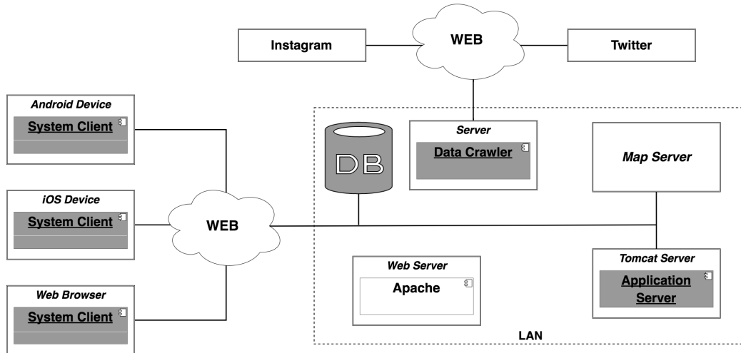
Figure 1: VazaDengue architecture
