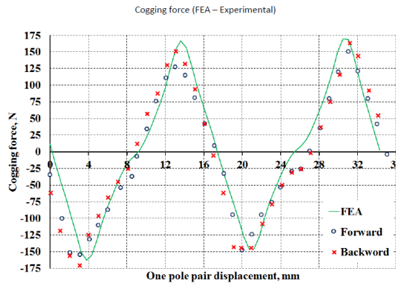
Figure 12: Predicted and measured cogging force
