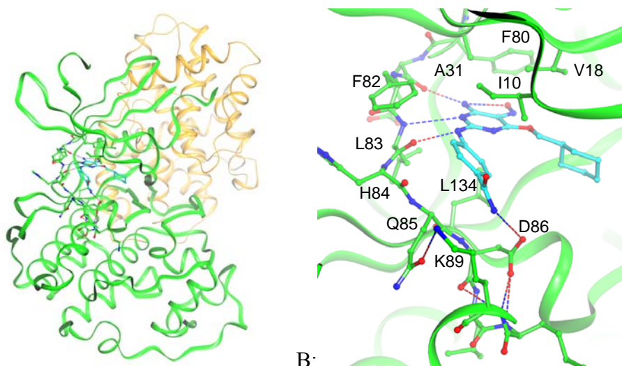
Figure 2: A: Crystal structure of 7j bound to Thr160pCDK2/cyclin A, overall fold. CDK2 and cyclin A are rendered in green and gold ribbons, respectively. Compound 7j occupies the ATP binding site and is drawn in ball and stick mode with carbon, nitrogen, and oxygen atoms coloured green, red, and blue, respectively. B: Compound 7j bound to the CDK2 active site. The side chains of selected residues that line the CDK2 active site are included. Hydrogen-bonds between 7j and CDK2 are drawn as dashed lines.
